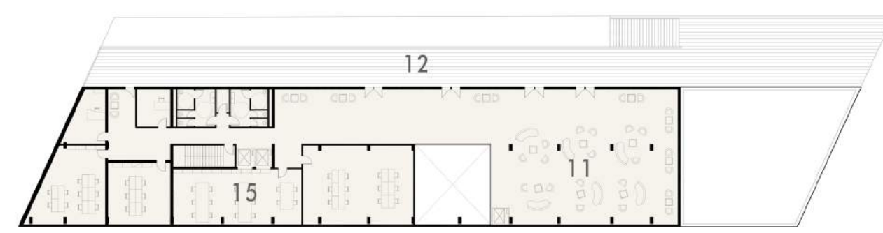
R+7 (+ 31.00M)
