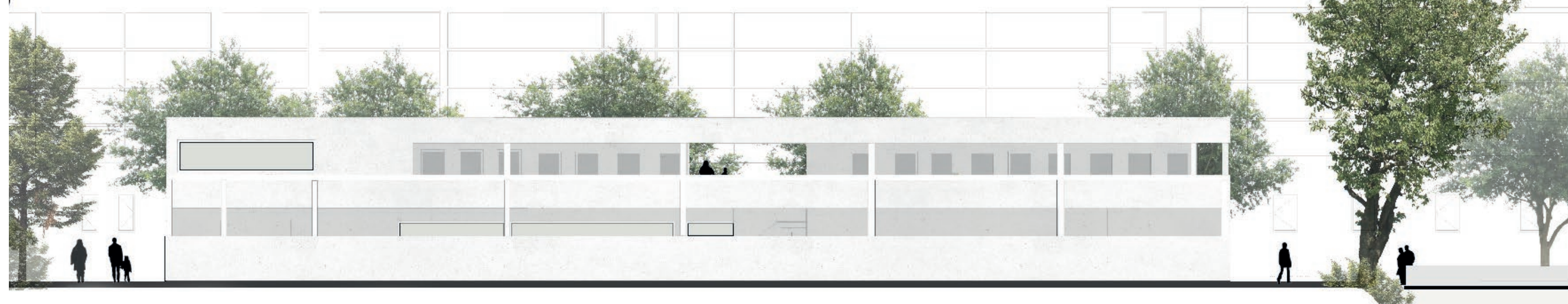
FACADE SUD
